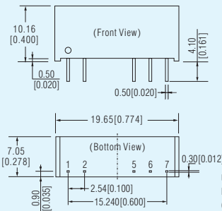
E_S-2WR2, F_S-2WR2, F_S-3WR2 Series(SIP) LxWxH: 19.65x7.05x10.16(mm)
