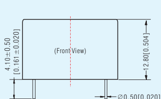
TDHx01D485H Series: LxWxH: 20.00X17.00X12.80(mm)
