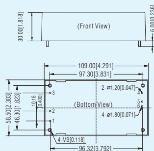
Pin-Out
