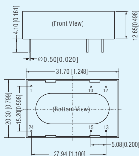
QAU242D2G: LxWxH: 31.70x20.30x12.65(mm)
