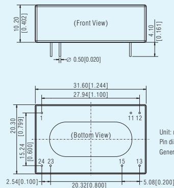
Package Dimension LxWxH: 31.60x20.30x10.20(mm)
