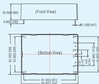
Pin-Out
