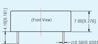
TDxx11D485H Series: LxWxH: 20.00X17.00X7.00(mm)
