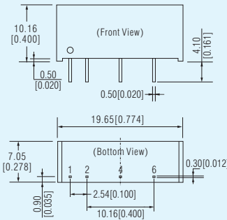
B_S-3WR2 Series (SIP) LxWxH: 19.65x7.05x10.16(mm)
