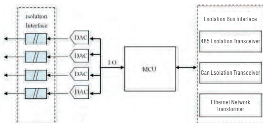
Fig 8. DCS System AO Interface Isolation Application
