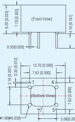
F05_N-1WR3 Series (DIP) LxWxH: 12.70x10.16x8.20(mm)
