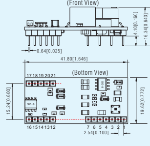
TLAxx-03KCAN Series; LxWxH: 41.80x19.62x16.34(mm)
