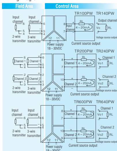
Wiring Diagram
