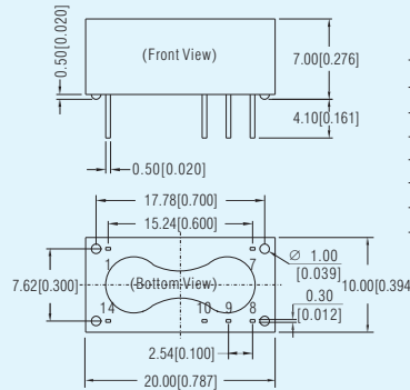
E/F_D-1WR2、E_D-1WR3 Series (DIP) LxWxH: 20.00x10.00x7.00(mm)
