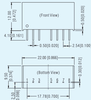
Package Dimension LxWxH: 22.00x9.50x12.00(mm)
