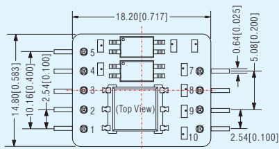
TD5(3)21S485x Series: LxWxH: 18.20X14.80X7.10(mm)
