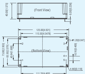
Pin-Out
