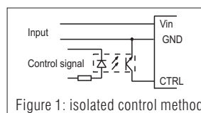
Figure 1: isolated control method
