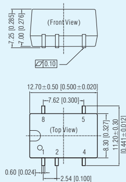
B/F_XT-2WR2 Series LxWxH: 12.70x11.20x7.25(mm)
