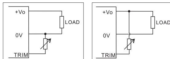
Figure 1: How to connect resistors for trimming
